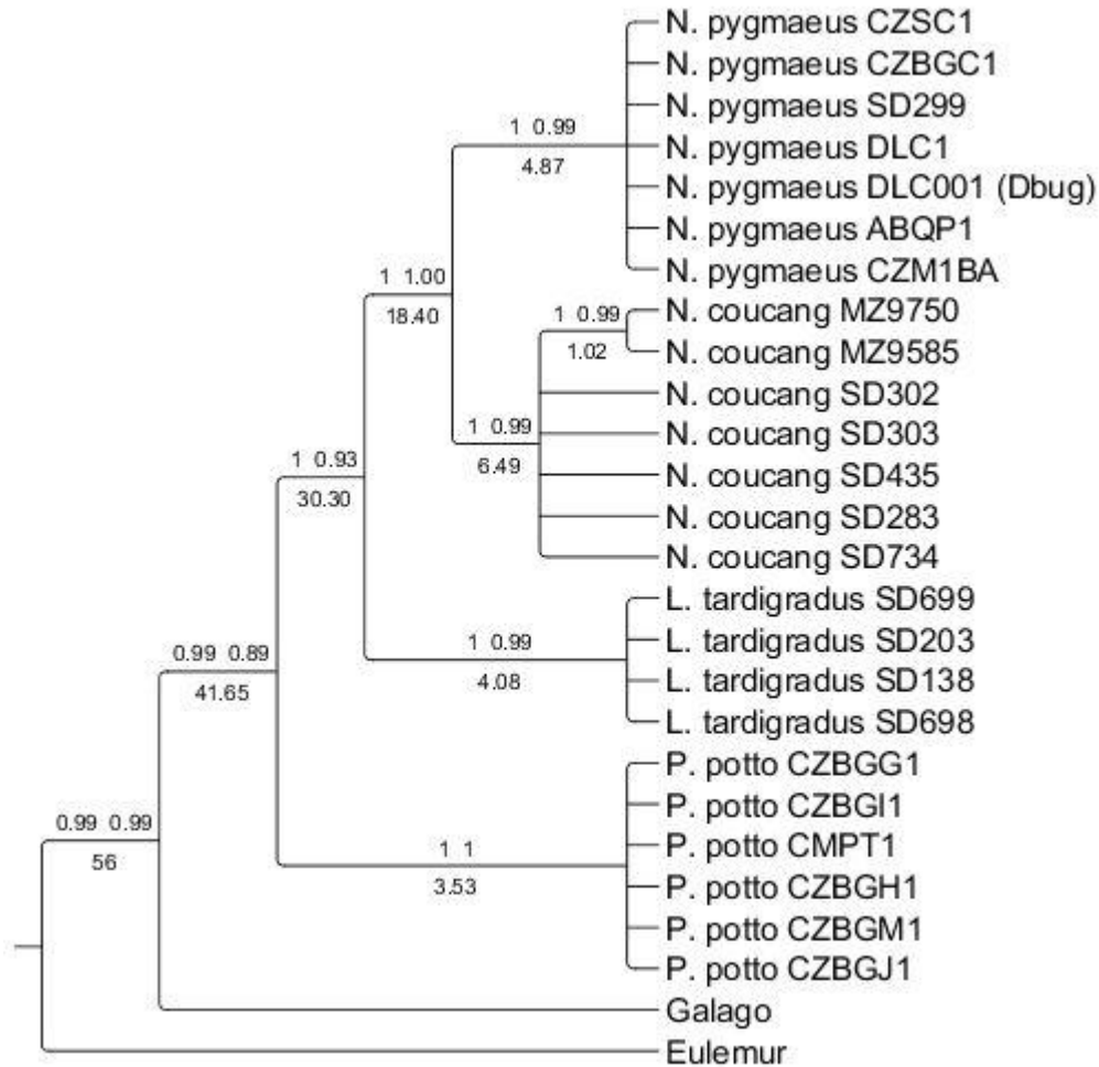
Figure 2: Monophyletic Lorisidae phylogeny based on concatenated genes. Numbers below branches are the divergence date in million years of the node. Numbers on top of the branches to the left are the Bayesian posterior probability, and numbers to the right are the Maximum Likelihood bootstrap probability for the node.
