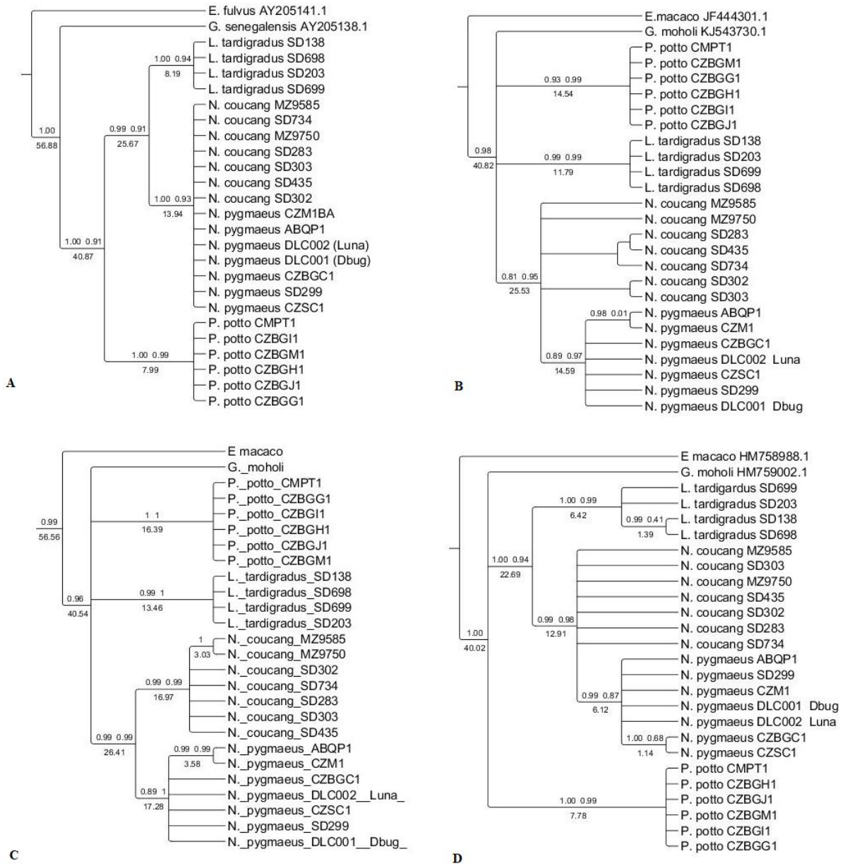
Figure 4: Lorisidae phylogenies from Mc1r (A), COI (B), concatenated mtDNA (C), and Rag2 without Arctocebus (D). Support values on branches are the same as Figure 1.
