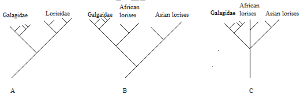
Figure 1: Commonly proposed loris phylogenies: (A) shows a monophyletic loris (Lorisidae) grouping, (B) shows a geographically parsimonious African and Asian grouping (a less parsimonious alternative is Asian lorises are more closely related to galagos-not shown), (C) indicates that Galagidae, the African, and the Asian lorises are all equally related.
