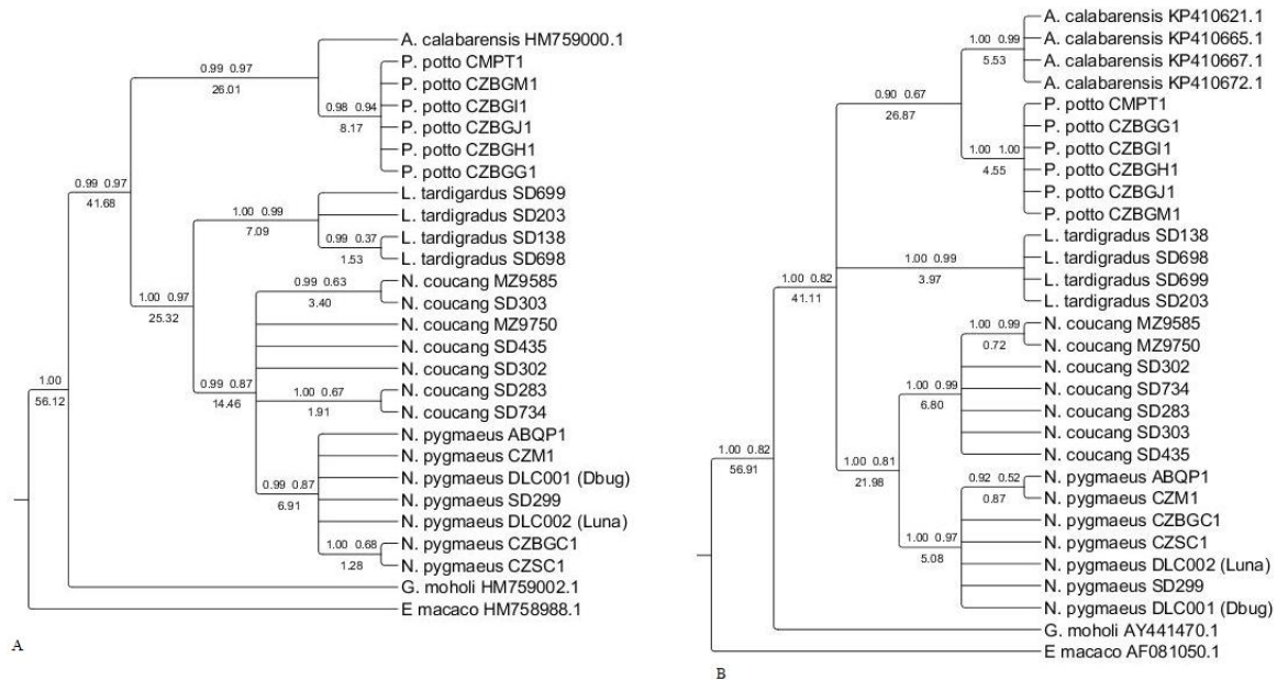
Figure 3: Lorisidae phylogenies from Rag2 (A) and cytochrome b (B) with Arctocebus sequences. Support values on branches are the same as Figure 1.
